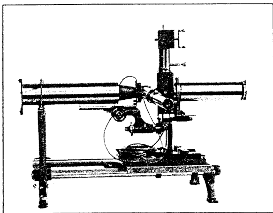
TEMPERATURE-CONTROLLED APPARATUS.
